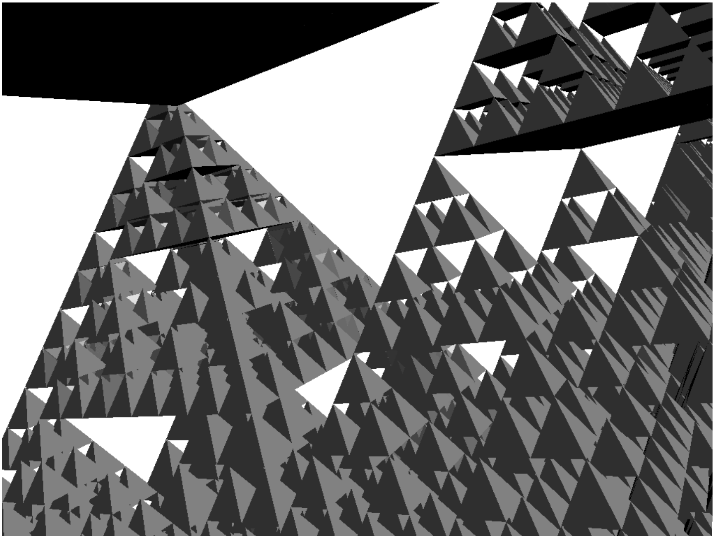
Sierpinski's Gasket in 3D.
